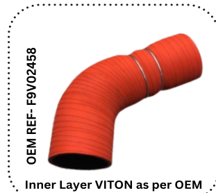
IKO - HUMP - 044 Leyland L-Bend Hump Hose "2 1/2" * "11" Long (2 Ring)
